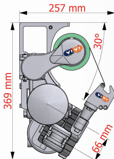
Vista Tenda 30°:
